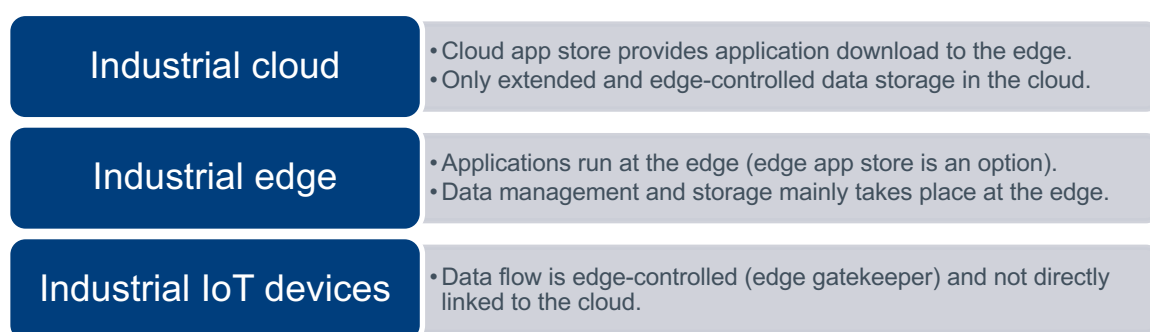
Fig. 8: Basic aspects of the industrial edge concept
