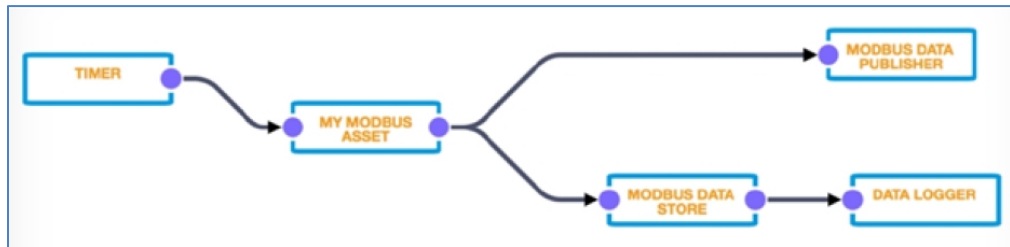
Figure 3. Wires components simplify the programming aspects of integrating sensors, actuators and other OT products.
