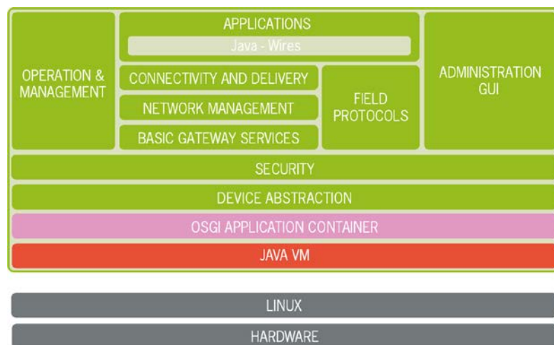
Figure 8. ESF enables wide, deep, seamless integration of applications with the operating system (Linux) and the hardware (devices), while providing full flexibility in terms of programming.
