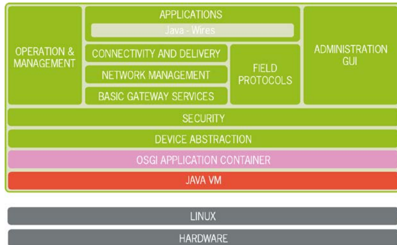
Figure 1. ESF enables wide, deep, seamless integration of applications with the operating system (Linux) and the hardware (devices), while providing full flexibility in terms of programming.
