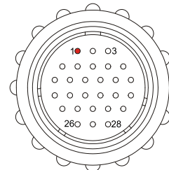
Cn1: Male 28-Pin CPC
