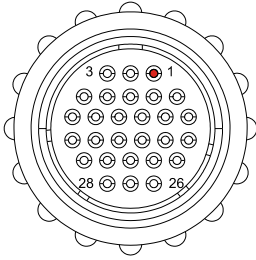
Cn1: Female 28-Pin CPC
