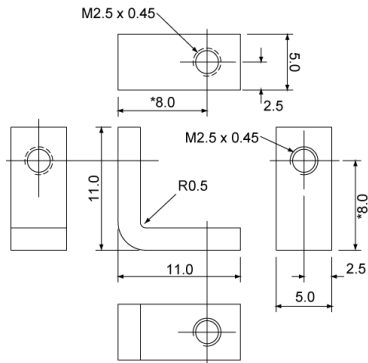
Mounting bracket dimensions (mm)
